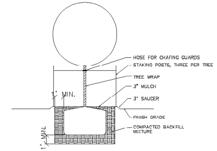
SECTION - TYPICAL TREE PLANTING DETAIL
