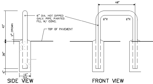
PUMP ISLAND PROTECTION BOLLARD
