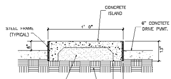
FUEL DISPENSING ISLAND SECTION
