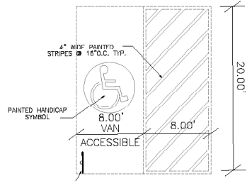
VAN ACCESSIBLE HANDICAP PARKING SPACE
