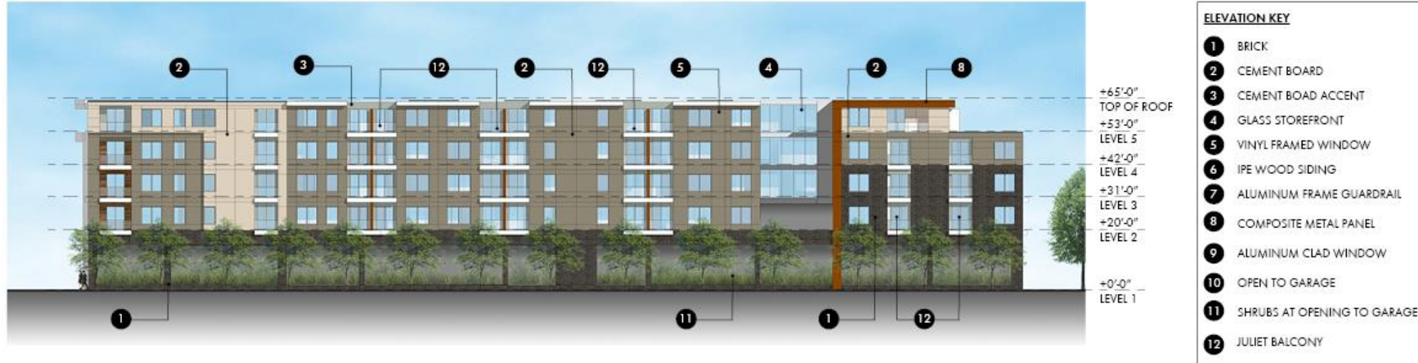
West Elevation
